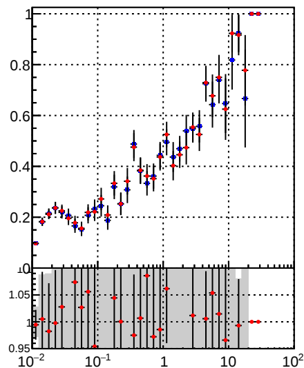
■ /data2/legianni/BDT-vs-DNN/real-BDT/CMSSW_13_0_0_pre4/src/runrem/DQM_TT_mkFit_ ● DQM_TT_mkFitRETEST_
