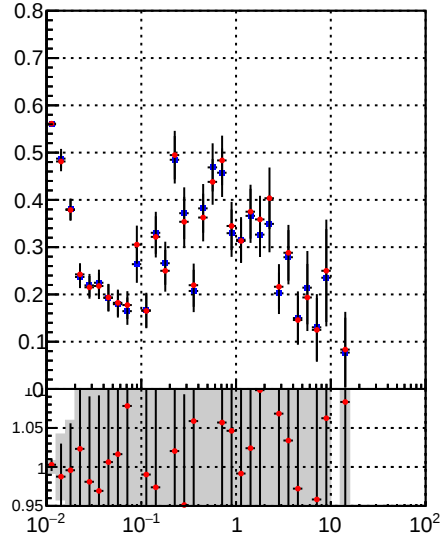
■ /data2/legianni/BDT-vs-DNN/real-BDT/CMSSW_13_0_0_pre4/src/runrem/DQM_TT_mkFit_ ● DQM_TT_mkFitRETEST_
