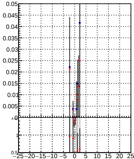
—●— /data2/legianni/BDT-vs-DNN/real-BDT/CMSSW_13_0_0_pre4/src/runrem/DQM_TT_mkFit_ —●— DQM_TT_mkFitRETEST
