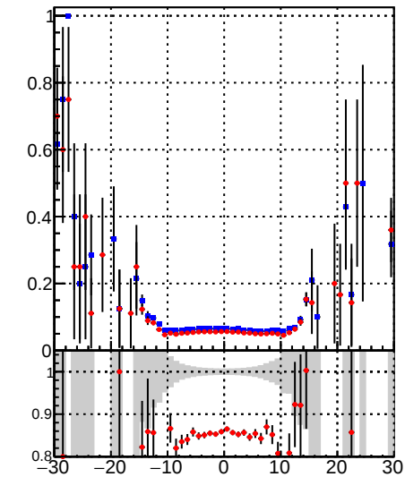
—●— /data2/legianni/BDT-vs-DNN/real-BDT/CMSSW_13_0_0_pre4/src/runrem/DQM_TT_mkFit_ —●— DQM_TT_mkFitRETEST
