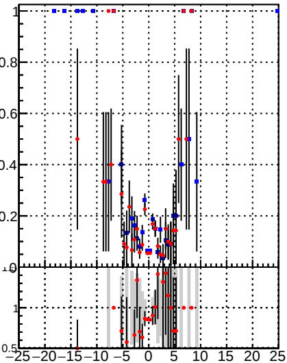
—●— /data2/legianni/BDT-vs-DNN/real-BDT/CMSSW_13_0_0_pre4/src/runrem/DQM_TT_mkFit_ —●— DQM_TT_mkFitRETEST
