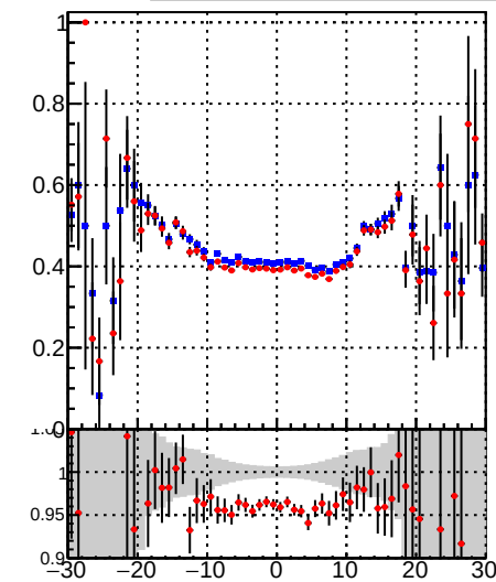
/data2/legianni/BDT-vs-DNN/real-BDT/CMSSW_13_0_0_pre4/src/runrem/DQM_TT_mkFit_ DQM_TT_mkFitRETEST_
