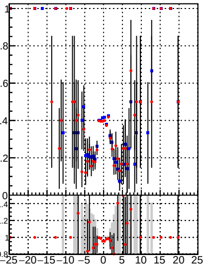
— /data2/legianni/BDT-vs-DNN/real-BDT/CMSSW_13_0_0_pre4/src/runrem/DQM_TT_mkFit_ — DQM_TT_mkFitRETEST
