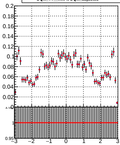
Legend: DQM_TT_mkFit-DQM_ DQM_TT_mkFit-DQM_adjusted
