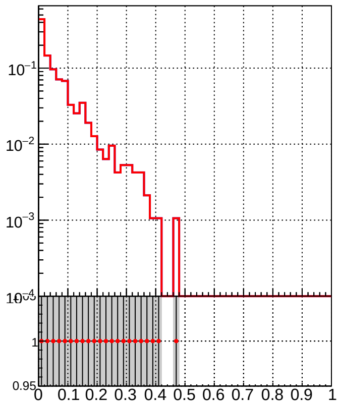
RecoPVAssoc2GenPVMatched_Missing
