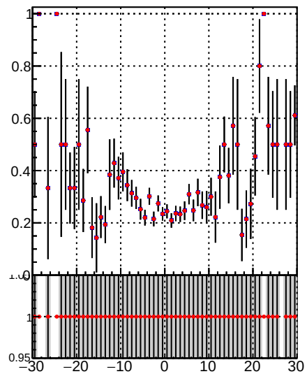
Fake rate vs \Delta
