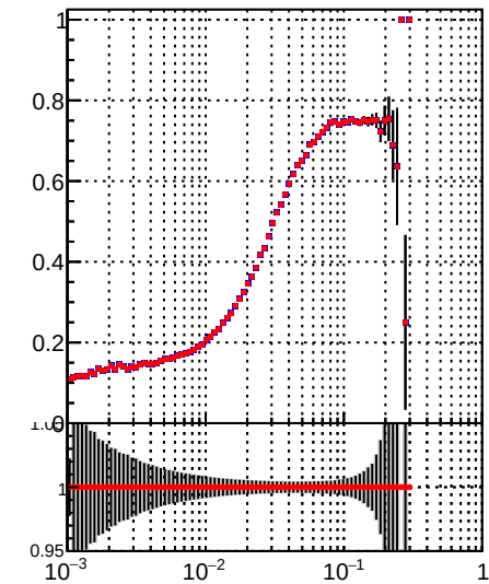
Fake rate vs \sqrt{s} Legend: DQM_TT_mkFit-DQM_ (black line with error bars) DQM_TT_mkFit-DQM_adjusted (red line with error bars)
