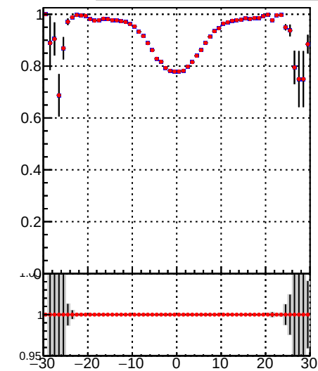
—•— DQM_TT_mkFit-DQM_ —•— DQM_TT_mkFit-DQM_adjusted
