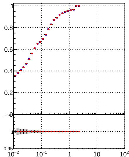
—•— DQM_TT_mkFit-DQM_ —•— DQM_TT_mkFit-DQM_adjusted
