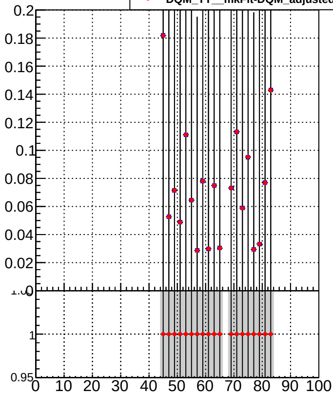
—•— DQM_TT_mkFit-DQM_ —•— DQM_TT_mkFit-DQM_adjusted
