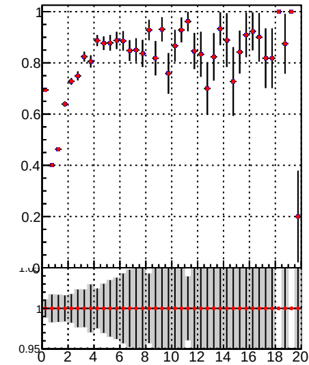
Fake rate vs. DQM TT mkFit-DQM DQM TT mkFit-DQM adjusted
