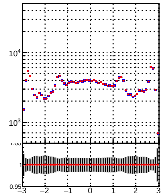
—●— DQM_TT_mkFit-DQM_ —●— DQM_TT_mkFit-DQM_adjusted
