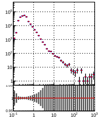
—●— DQM_TT_mkFit-DQM_ —●— DQM_TT_mkFit-DQM_adjusted
