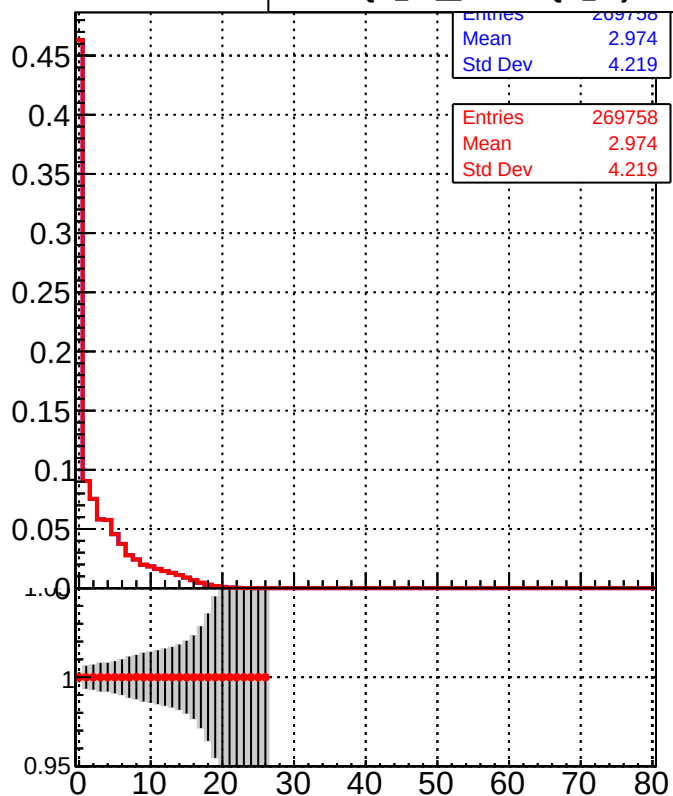
Legend: DQM_TT_mkFit-DQM_ (grey bars) DQM_TT_mkFit-DQM_adjusted (red line)
