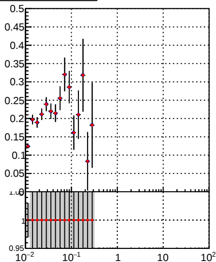
█ DQM_TT_mkFit-DQM_ ● DQM_TT_mkFit-DQM_adjusted
