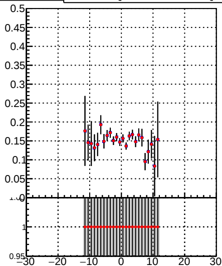
█ DQM_TT_mkFit-DQM_ ● DQM_TT_mkFit-DQM_adjusted
