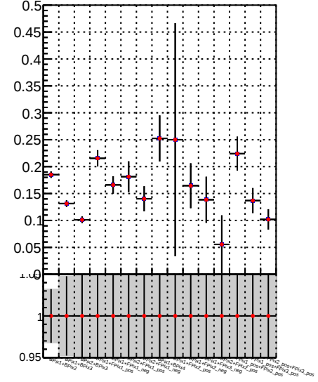
Fake rate vs. \square DQM TT mkFit-DQM \bullet DQM TT mkFit-DQM adjusted
