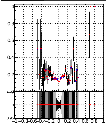
—●— DQM_TT_mkFit-DQM_ —●— DQM_TT_mkFit-DQM_adjusted
