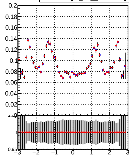
■ \text{DQM\_TT\_mkFit-DQM\_} ◆ \text{DQM\_TT\_mkFit-DQM\_adjusted}
