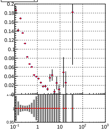
■ \text{DQM\_TT\_mkFit-DQM\_} ◆ \text{DQM\_TT\_mkFit-DQM\_adjusted}
