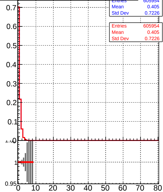
Legend: DQM_TT_mkFit-DQM_ (grey histogram), DQM_TT_mkFit-DQM_adjusted (red line)
