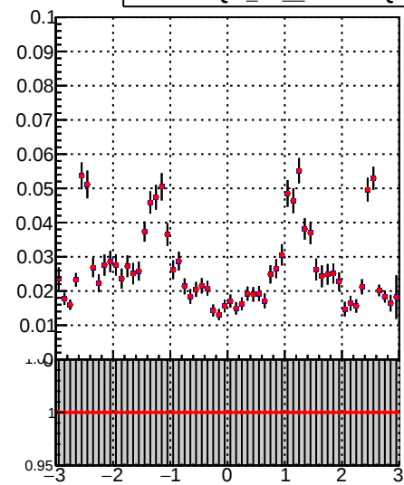
—•— DQM_TT_mkFit-DQM_ —•— DQM_TT_mkFit-DQM_adjusted
