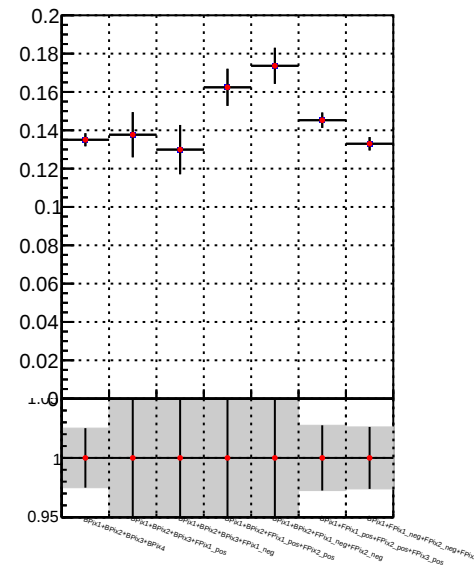
Fake rate vs. DQM_TT_mkFit-DQM DQM_TT_mkFit-DQM_adjusted
