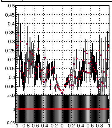
Efficiency vs DQM_TT_mkFit-DQM_
