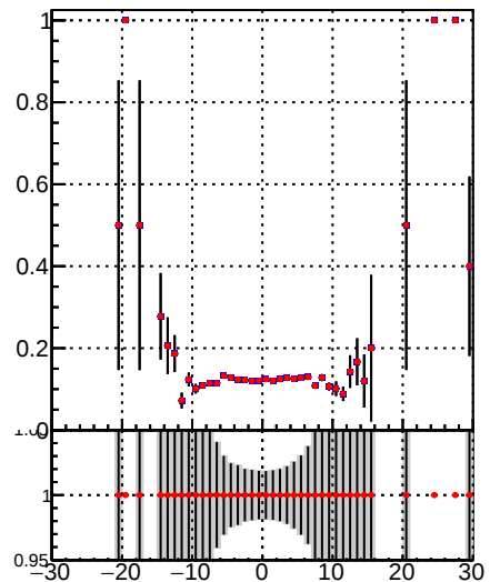
—•— DQM_TT_mkFit-DQM_ —•— DQM_TT_mkFit-DQM_adjusted
