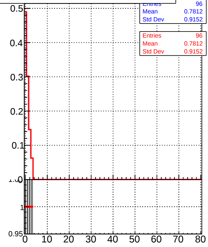
Legend: DQM_TT_mkFit-DQM_ (blue line with squares), DQM_TT_mkFit-DQM_adjusted (red line with circles)
