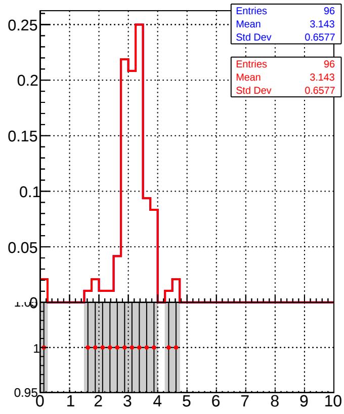
Legend: DQM_TT_mkFit-DQM_ (blue line with squares), DQM_TT_mkFit-DQM_adjusted (red line with circles)
