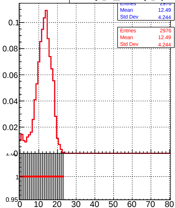
DQM_TT_mkFit-DQM_ DQM_TT_mkFit-DQM_adjusted
