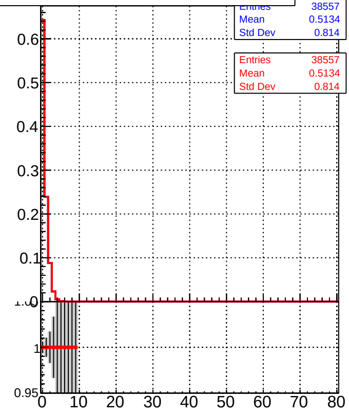
DQM_TT_mkFit-DQM_ DQM_TT_mkFit-DQM_adjusted
