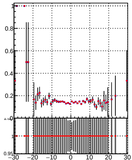
Fake rate vs d —•— DQM TT mkFit-DQM —•— DQM TT mkFit-DQM_adjusted
