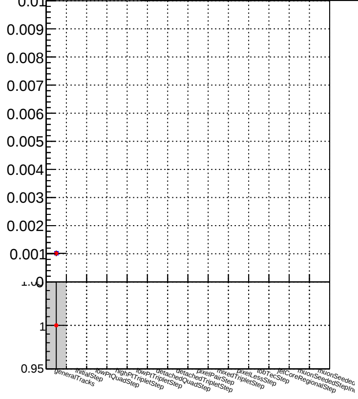
Duplicates rate vs collection Legend: DQM_TT_mkFit-DQM_ (Blue square) DQM_TT_mkFit-DQM_adjusted (Red circle)
