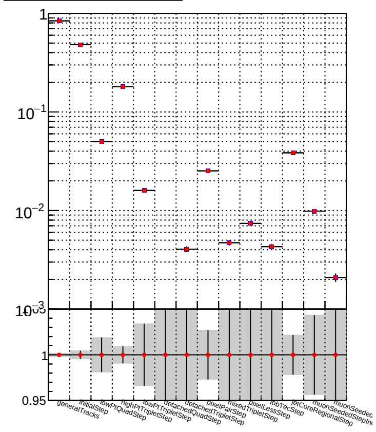
Duplicates rate vs collection Legend: DQM_TT_mkFit-DQM_ (Blue square) DQM_TT_mkFit-DQM_adjusted (Red circle)
