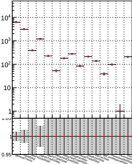
Number —●— DQM_TT_mkFit-DQM_adjusted
