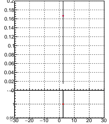
DQM_TT_mkFit-DQM_ DQM_TT_mkFit-DQM_adjusted
