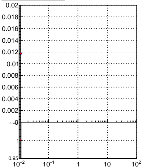
DQM_TT_mkFit-DQM_ DQM_TT_mkFit-DQM_adjusted
