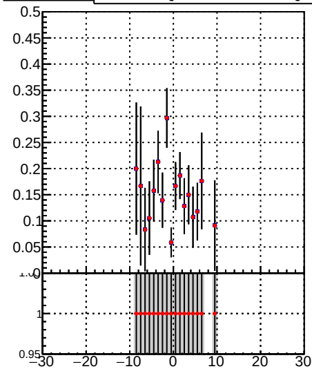
Fake rate vs v Legend: DQM_TT_mkFit-DQM_ DQM_TT_mkFit-DQM_adjusted
