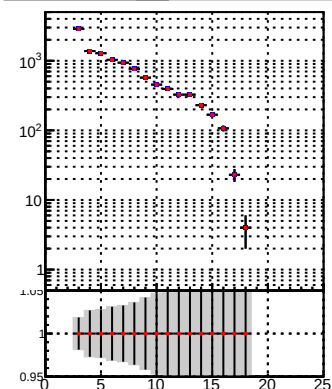
DQM_TT_mkFit-DQM_ DQM_TT_mkFit-DQM_adjusted
