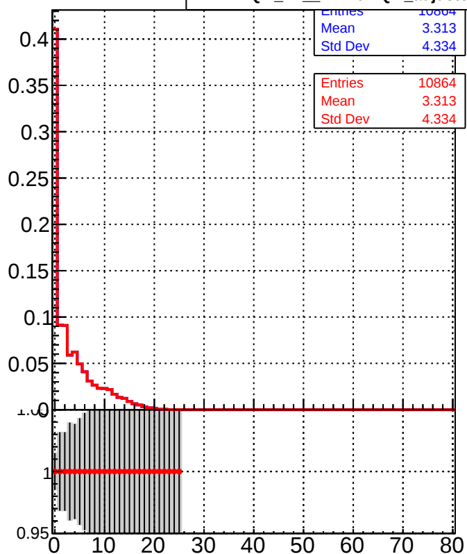
Legend: DQM_TT_mkFit-DQM_ (Blue line with markers) DQM_TT_mkFit-DQM_adjusted (Red line with markers)
