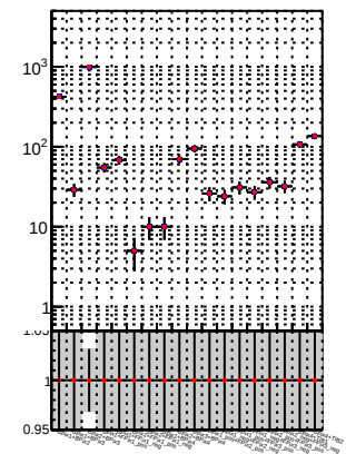
N of reco track vs. \chi^2 DQM TT mkFit-DQM DQM TT mkFit-DQM_adjusted
