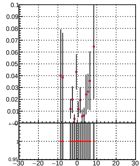
—•— DQM_TT_mkFit-DQM —•— DQM_TT_mkFit-DQM_adjusted
