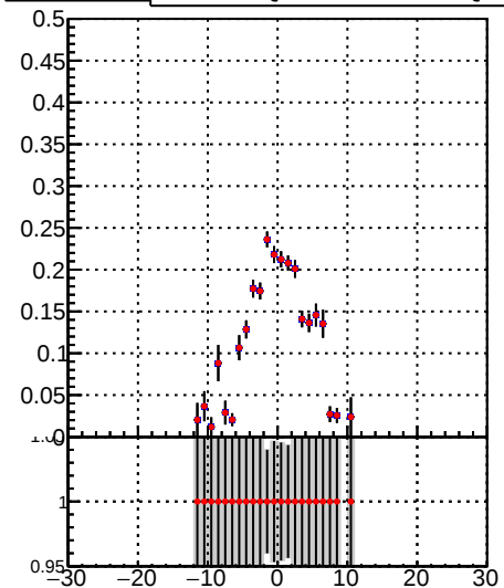
Fake rate vs \eta DQM_TT_mkFit-DQM_ DQM_TT_mkFit-DQM_adjusted
