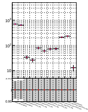
N of reco track vs. \chi^2 — DQM TT mkFit-DQM adjusted
