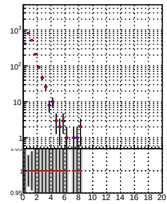
N of reco track vs. \chi^2 — DQM TT mkFit-DQM adjusted
