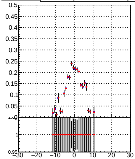
Fake rate vs \nu DQM_TT_mkFit-DQM_ DQM_TT_mkFit-DQM_adjusted
