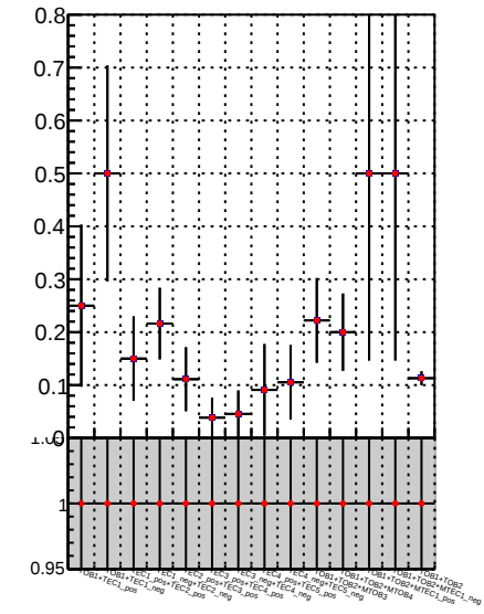
Fake rate vs. \square DQM_TT_mkFit-DQM \bullet DQM_TT_mkFit-DQM_adjusted
