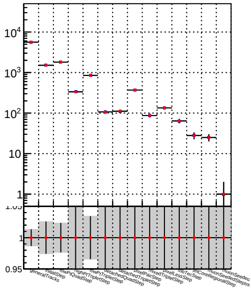
Number —●— DQM_TT_mkFit-DQM_adjusted
