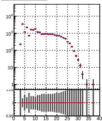
N of reco track vs hit DQM_TT_mkFit-DQM_ DQM_TT_mkFit-DQM_adjusted
