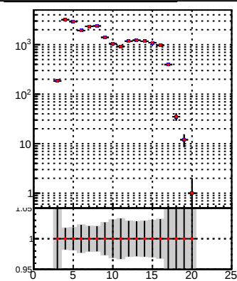
N of reco track vs hit DQM_TT_mkFit-DQM_ DQM_TT_mkFit-DQM_adjusted
