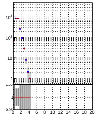
N of reco track vs. \chi^2 (mkFit-DQM vs. mkFit-DQM_adjusted)
