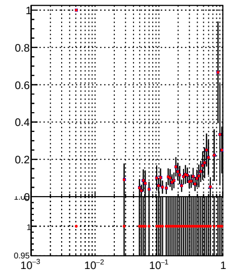
Fake rate vs \sqrt{s} DQM_TT_mkFit-DQM_ DQM_TT_mkFit-DQM_adjusted
