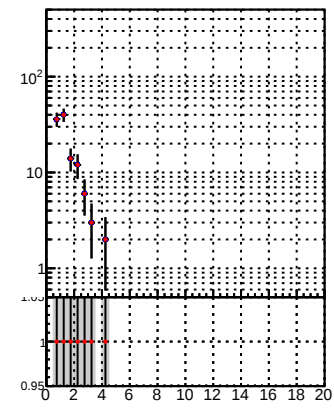
N of reco track vs. s DQM_TT_mkFit-DQM DQM_TT_mkFit-DQM_adjusted
