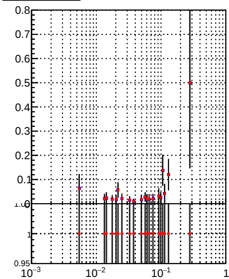
Fake rate vs \sqrt{s} DQM_TT_mkFit-DQM_ DQM_TT_mkFit-DQM_adjusted
