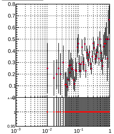
Legend: DQM_TT_mkFit-DQM_ DQM_TT_mkFit-DQM_adjusted
