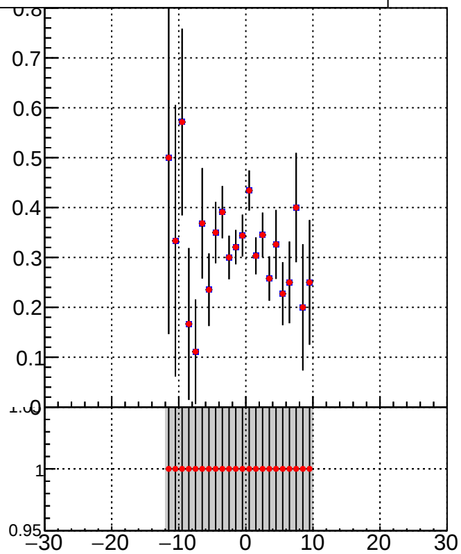
DQM_TT_mkFit-DQM_ DQM_TT_mkFit-DQM_adjusted
