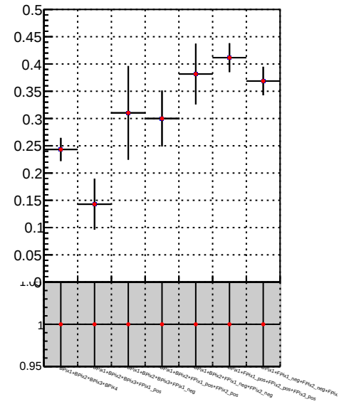
Fake rate vs. \square DQM_TT_mkFit-DQM \bullet DQM_TT_mkFit-DQM_adjusted
