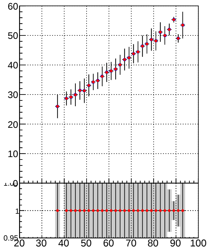
MatchedRecoVtx_vs_GenVtx
