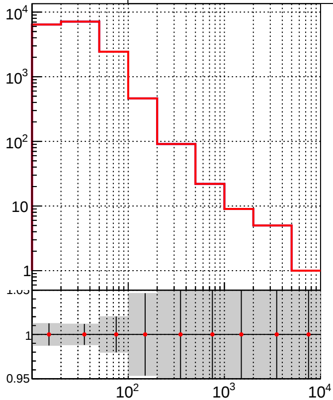
RecoAssoc2GenPVMatched_Pt2
