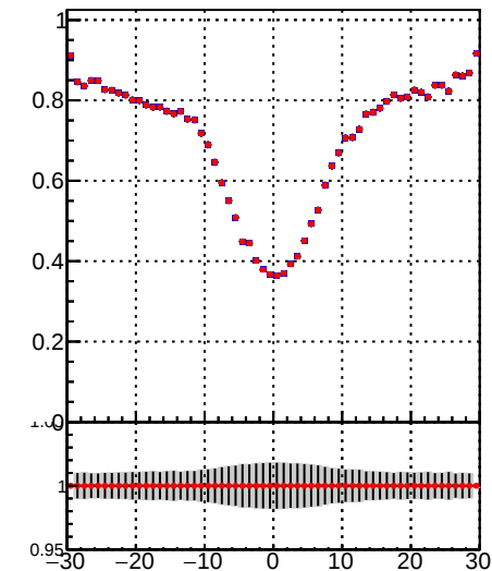
—•— DQM_TT_mkFit-DQM_ —•— DQM_TT_mkFit-DQM_adjusted
